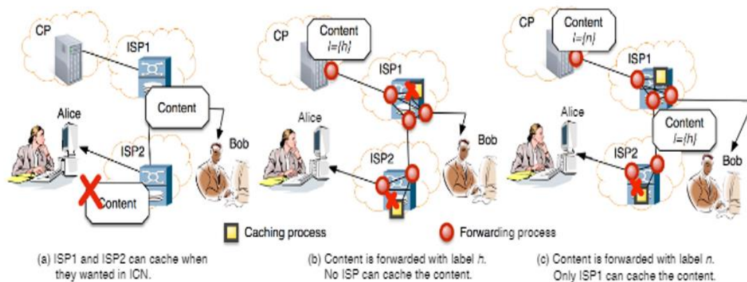
Figure 2.2. Different ISPs can have different permissions to cache contents
