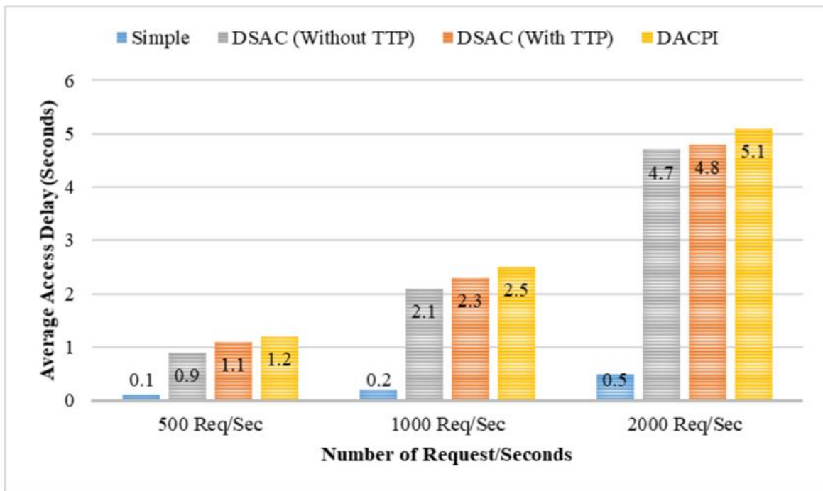
Figure 4.4 Average Access Delay (Seconds) of Simple, DSAC (Without TTP), DSAC (With TTP) and DACPI.
