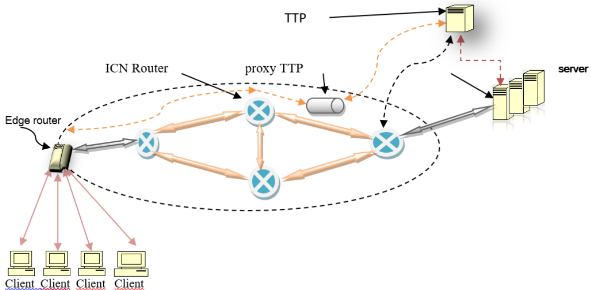
Figure 3.1 Digital Signature Cryptography Based encryption in ICN.
