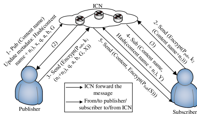
Figure 2.1 Decentralized access control protocol in ICN .
