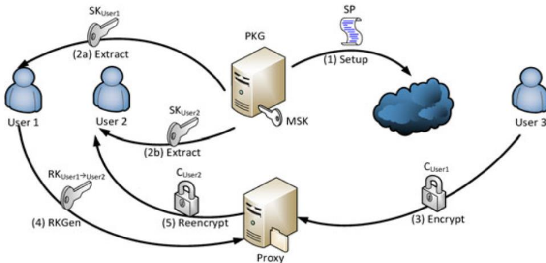
Figure 2.3. The IBE-PRE scheme of Ateniese and Green
