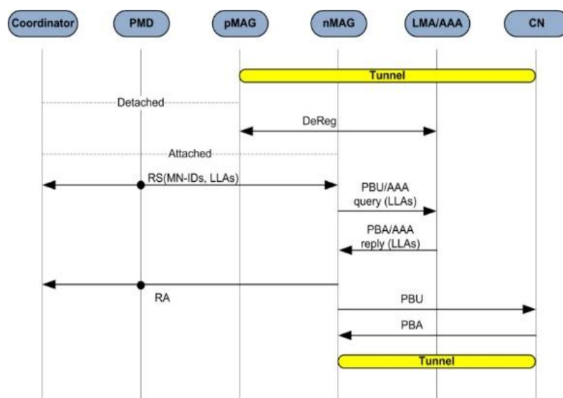
Figure 3 The signaling flow
